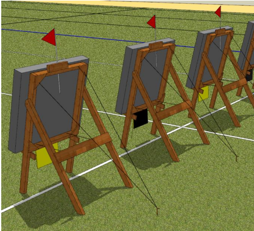
Figure 11. Target Buttress Rear View showing tie back
